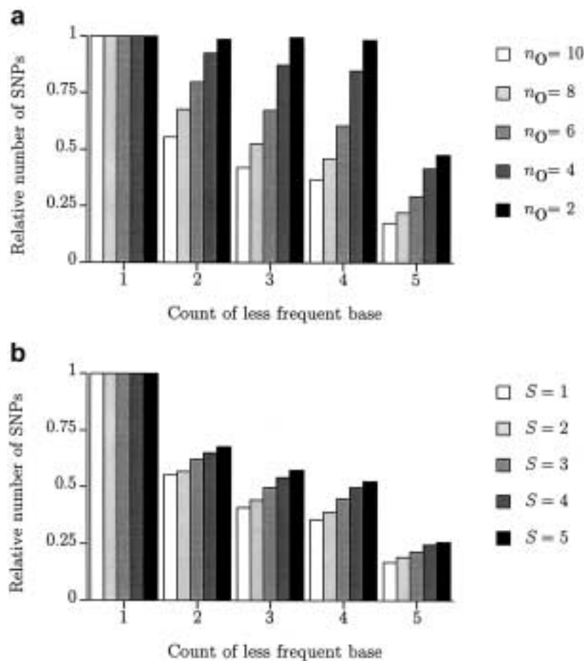
Figure 3 Expected numbers of SNPs segregating in different frequencies, in a sample of size n_A + n_O = 10 , relative to the number of singleton polymorphisms; results are averages, over 100,000 simulated data sets, for a 400-bp-long SDL, with \theta = .0005 per base pair. a , Effect of requiring an SDL to have at least one SNP in the first n_O samples drawn from the population. b , Effect of separating SDLs into classes with different numbers of SNPs, with n_D = 0 .
