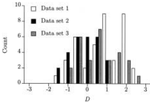
Figure 2 Distribution of Tajima's (1989) D among SDLs, in each of the three data sets.
