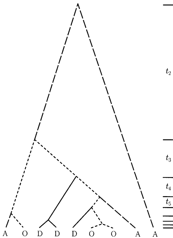
Figure 1 Example genealogy, drawn with branch lengths equal to the coalescent expectations, which shows the structure of the data analyzed here: “A,” “D,” and “O” are, respectively, samples that are only in the ascertainment set, samples that are only in the data set, and “overlap” samples (i.e., those which are in both the data set and the ascertainment set). Three types of branches are distinguished, corresponding to the three kinds of observable polymorphisms discussed in the text.
